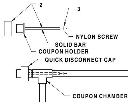
COUPON DETAIL
